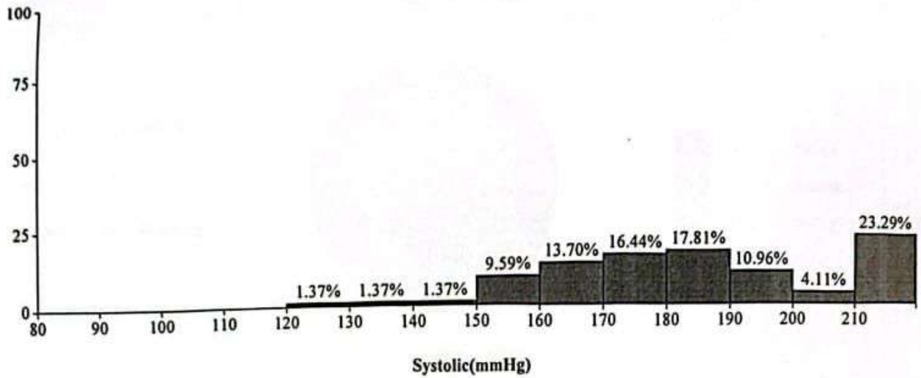
Histogram(All)
