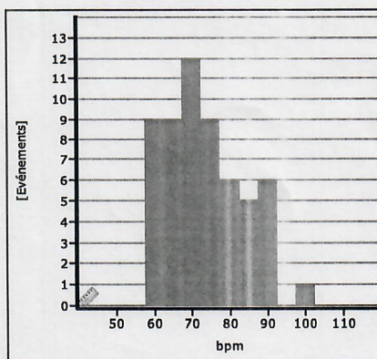
FC Total
