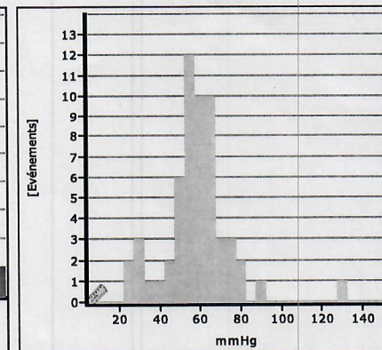
PP Total
