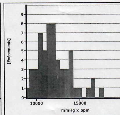
RPP Total
